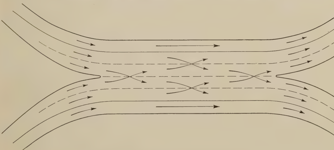
Figure 44.—A compound weaving section.
